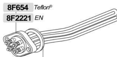
4GR 8F369 5000W 230V LSF=660mm 8F0368 5000W 380V LSF=660mm
